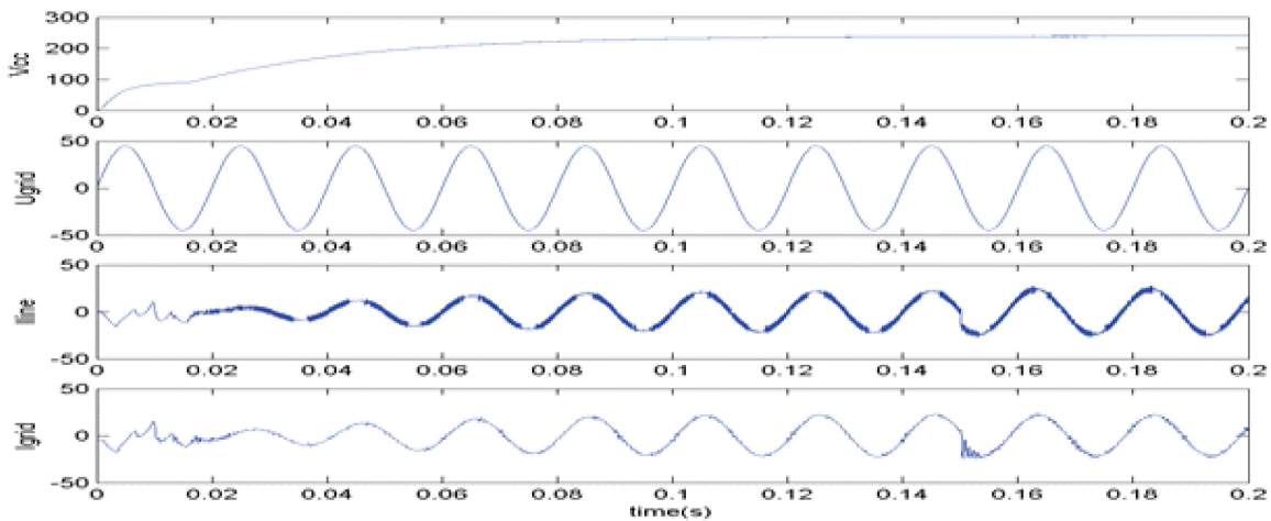
Fig. 3. Evolution of the main variables in the 3-phase grid connected system for phase 1
