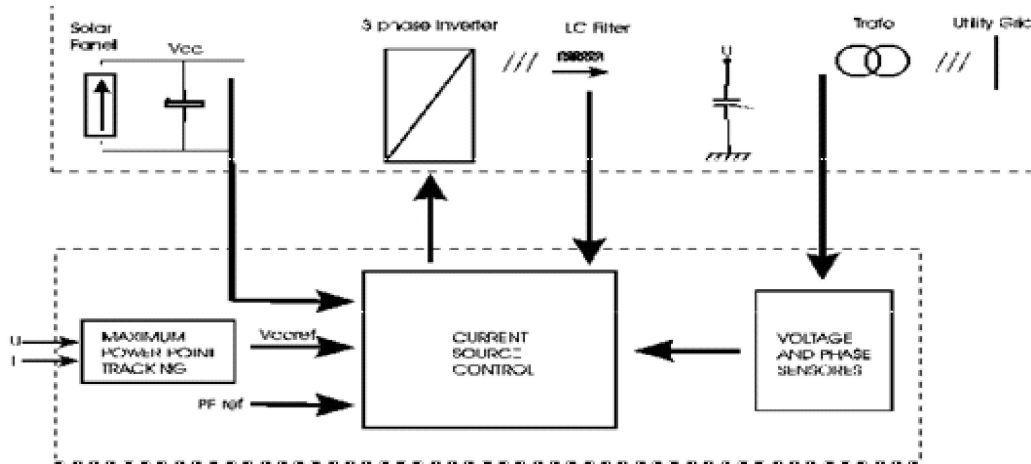
Fig. 1. Block diagram of the control of the grid-connected 3- phase inverter
