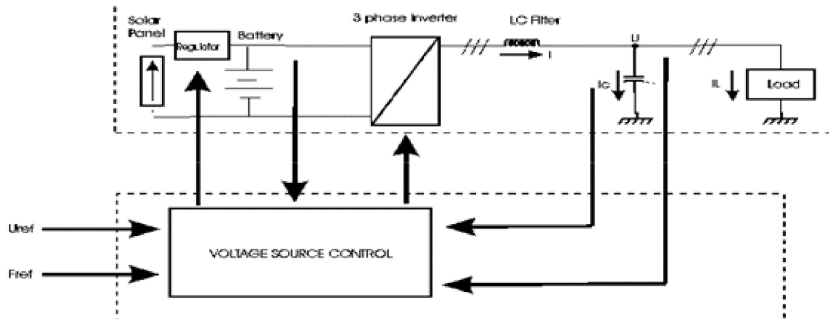
Fig. 2. Block diagram of the control of the 3-phase UPS system
