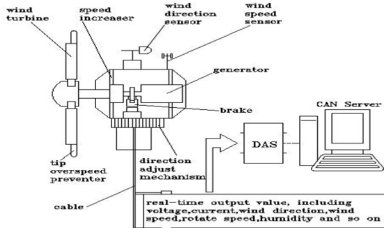
Fig.1: Monitoring and control of wind
