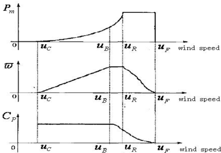
Figure 3 The three operation models of wind turbine Fig 4.: Doubly-fed generator
